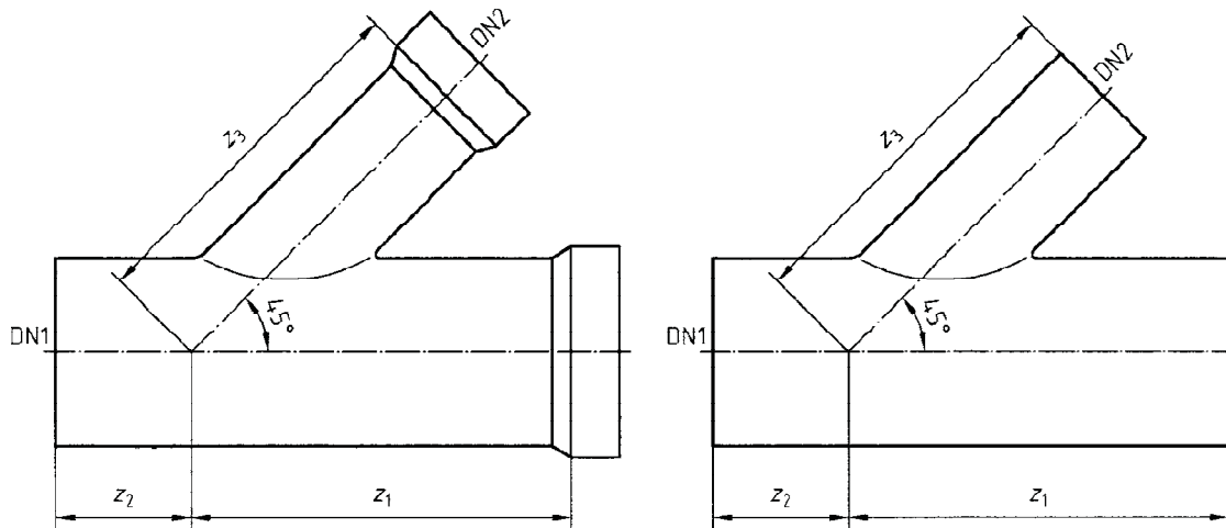
Figure 3: 45° branch
