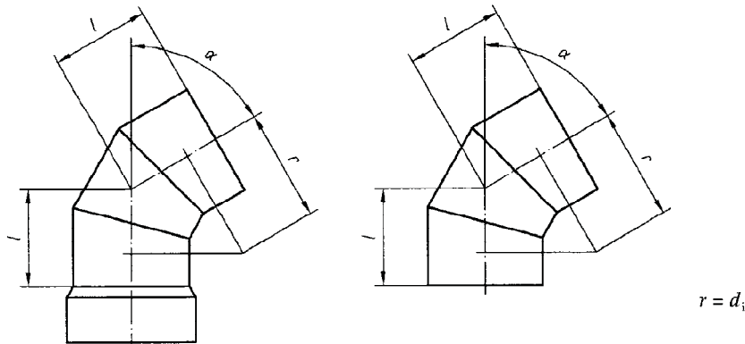
Figure 2: Gusseted bends
